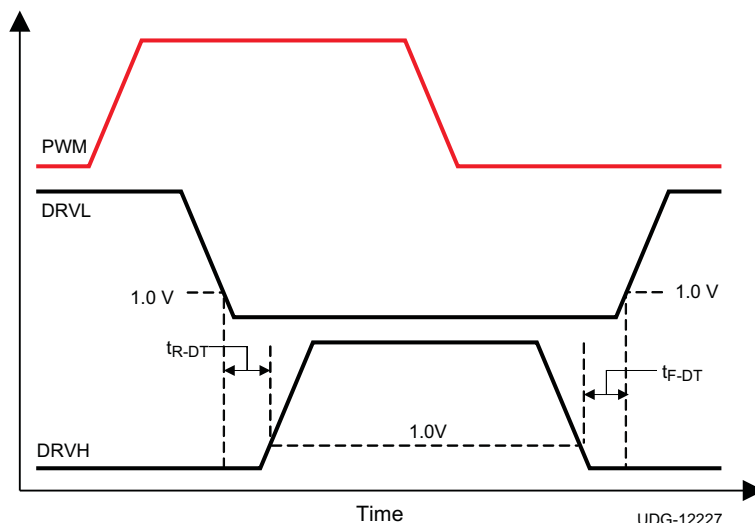
Figure 16. Dead-Time Definitions
