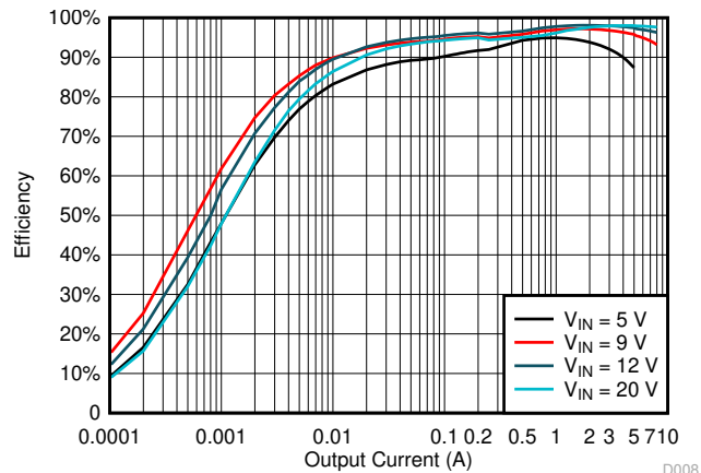
Figure 6-8. Efficiency vs Output Current, V_{OUT} = 15 V, PFM
