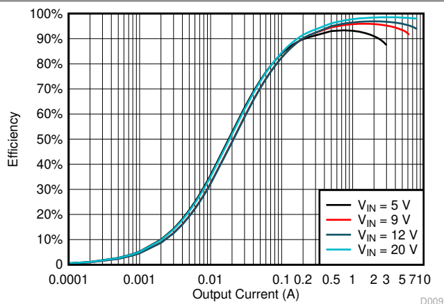
Figure 6-9. Efficiency vs Output Current, V_{OUT} = 20 V, FPWM
