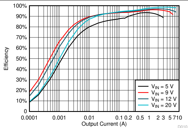
Figure 6-10. Efficiency vs Output Current, V_{OUT} = 20 V, PFM
