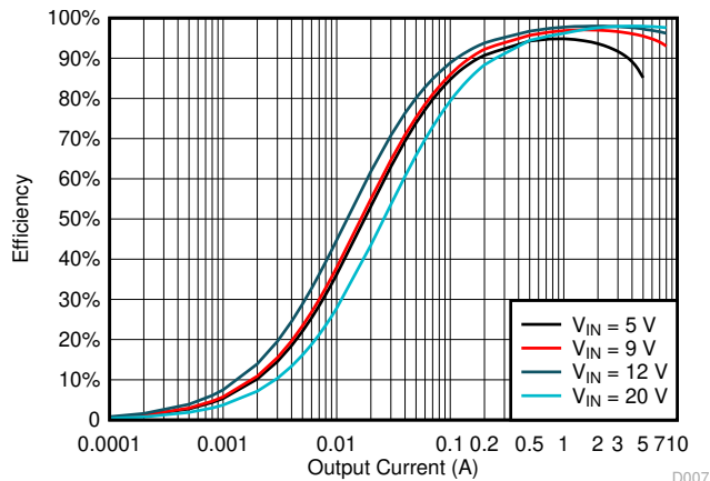
Figure 6-7. Efficiency vs Output Current, V_{OUT} = 15 V, FPWM
