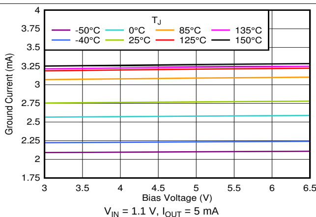
Figure 29. Quiescent Current vs Bias Voltage
