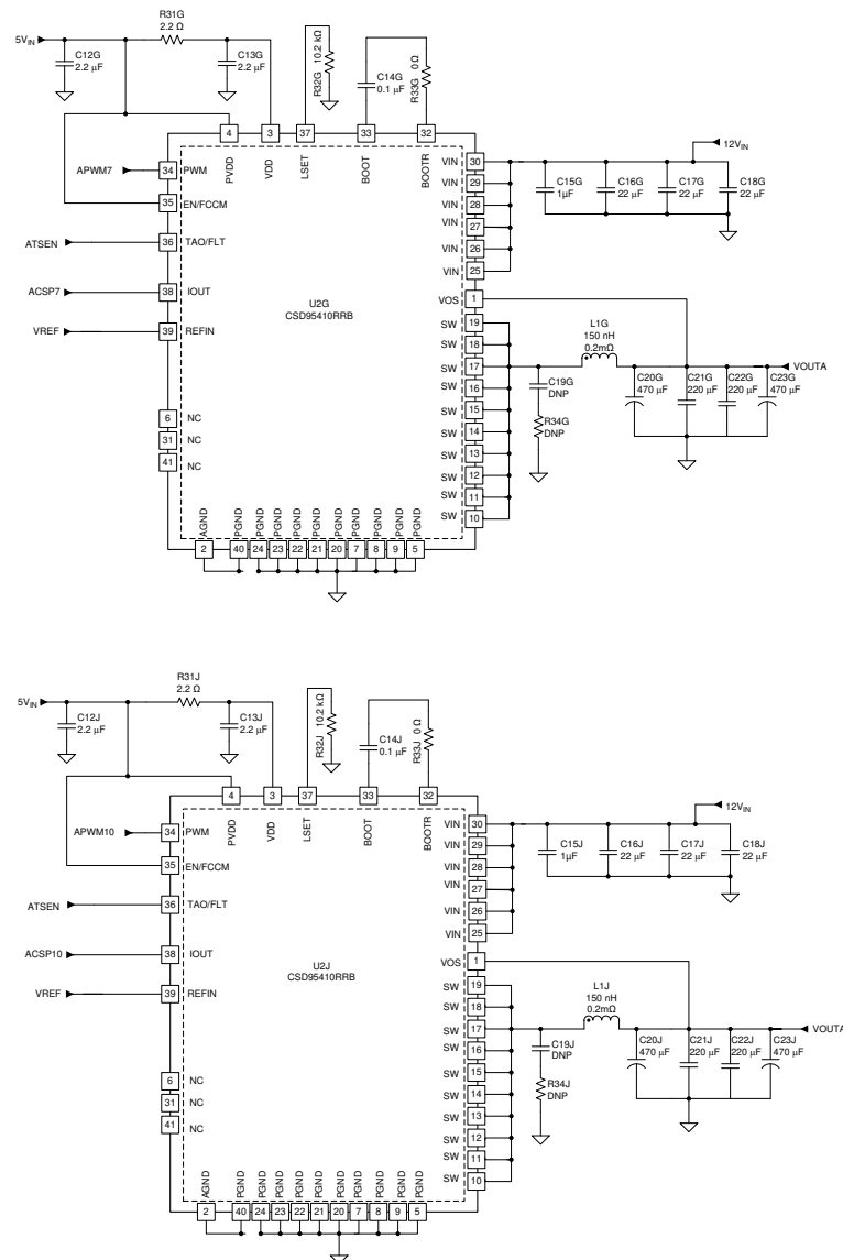
Figure 8-3. Powerstages Schematic (2/3)
