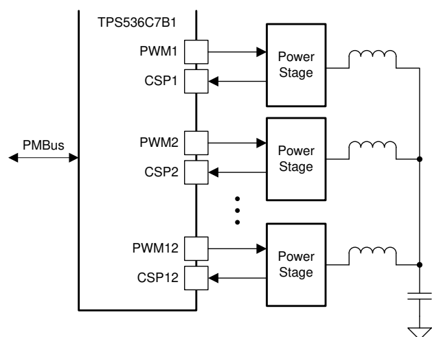
Simplified Schematic
