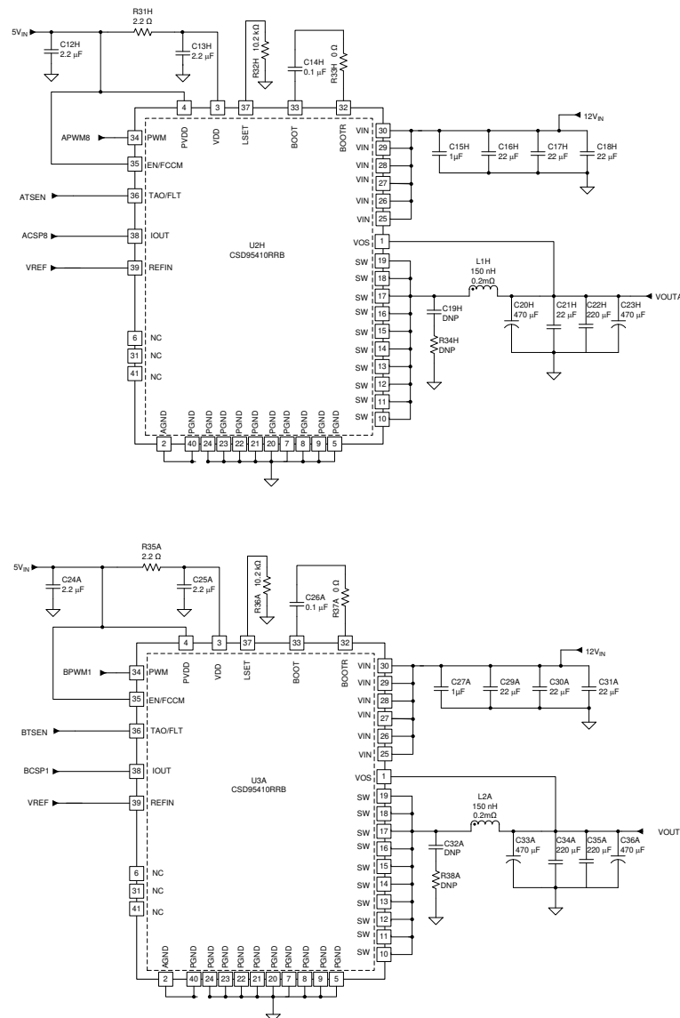
Figure 8-3. Powerstages Schematic (2/3)
