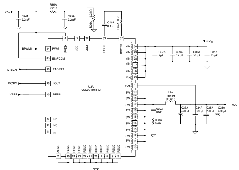
Figure 8-3. Powerstages Schematic (2/3)
