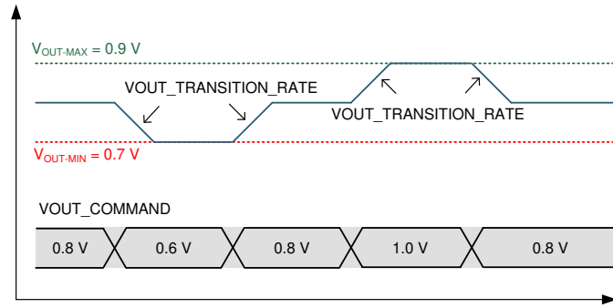
Figure 7-31. VOUT_MIN_MAX example
