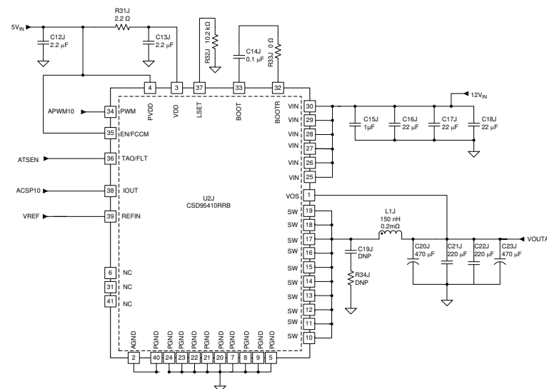
Figure 8-3. Powerstages Schematic (2/3)
