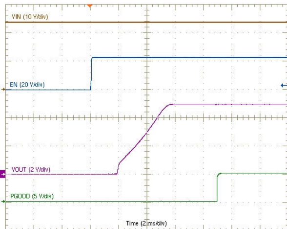
Figure 8-2. Start-Up Waveforms
