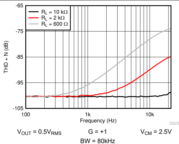
Figure 5-29. THD + N vs Frequency
