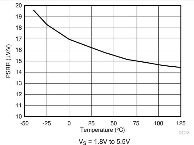
Figure 5-12. PSRR vs Temperature
