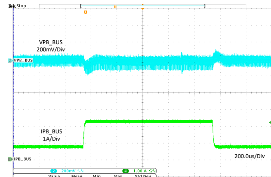
Figure 11-9. Load Transient Without Cable Compensation
