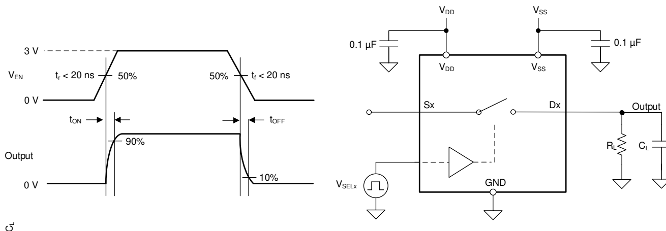
Figure 6-4. Turn-On and Turn-Off Time Measurement Setup
