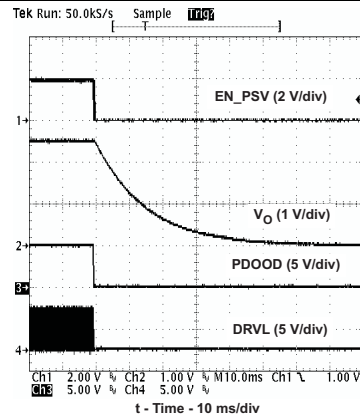
Figure 23. 2.5-V Shutdown Waveforms
