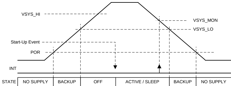
Figure 5-26. State Transitions
