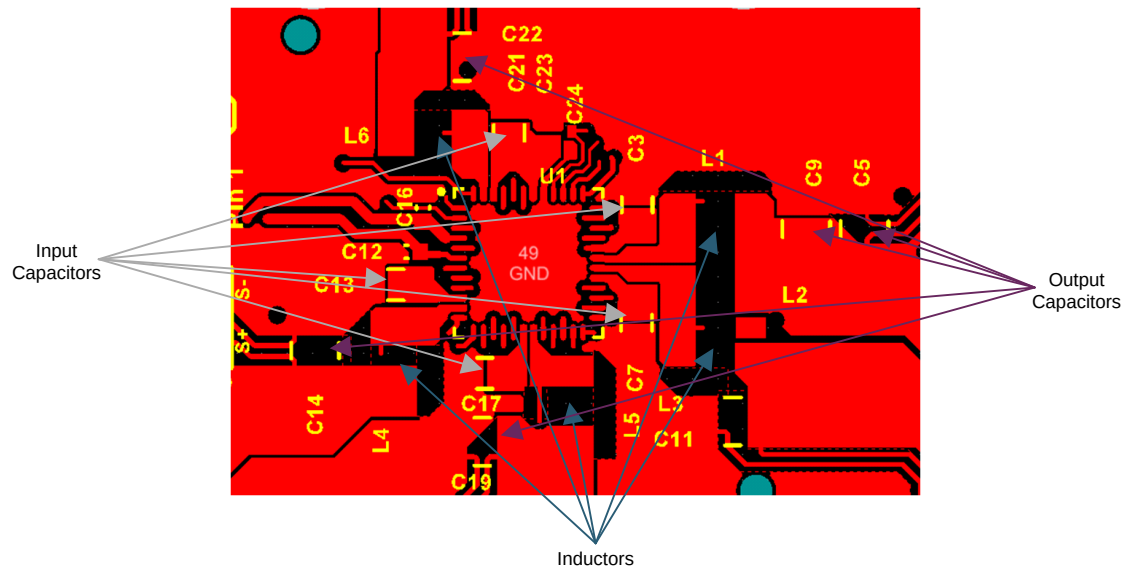
Figure 6-12. Top Layer Overview of Inductor and Capacitor Placement and Routing of SMPs
