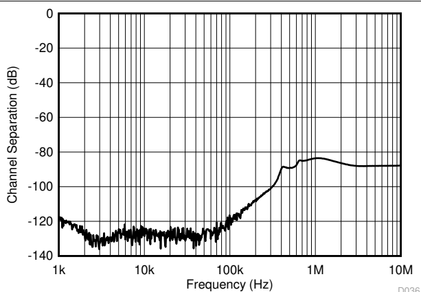
Figure 6-31. Channel Separation
