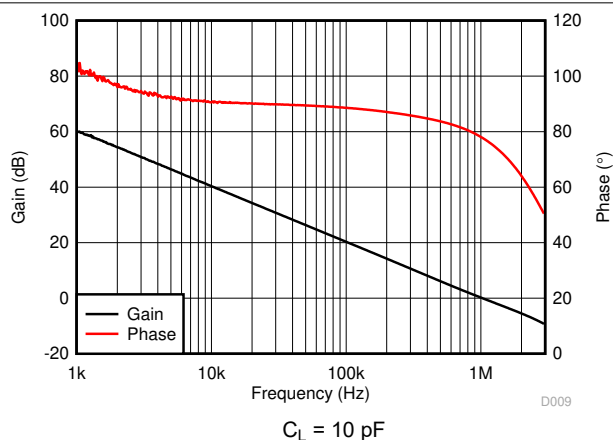
Figure 6-4. Open-Loop Gain and Phase vs Frequency
