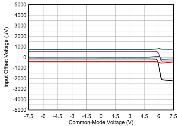
Figure 5-17. Input Offset Voltage vs Common-Mode Voltage
