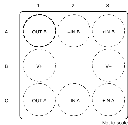
8-Bump DSBGA Package (Bump Side Down)—See Package Number YAF0008
