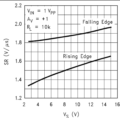
Figure 5-24. Slew Rate vs Supply Voltage
