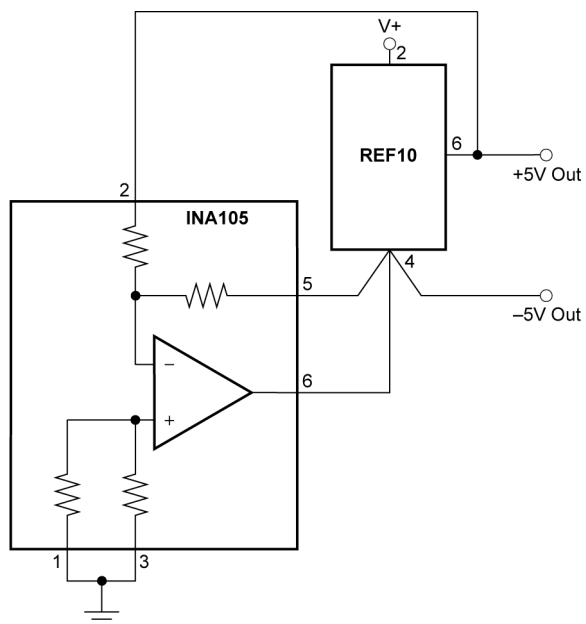
Figure 7-21. \pm 5\text{V} Precision Voltage Reference
