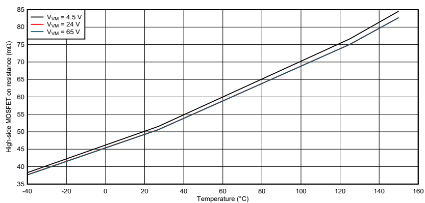
Figure 6-6. High-side FET on resistance
