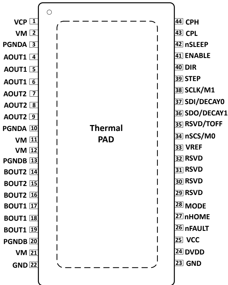
Figure 5-1. DDW Package (44-Pin HTSSOP), Top View
