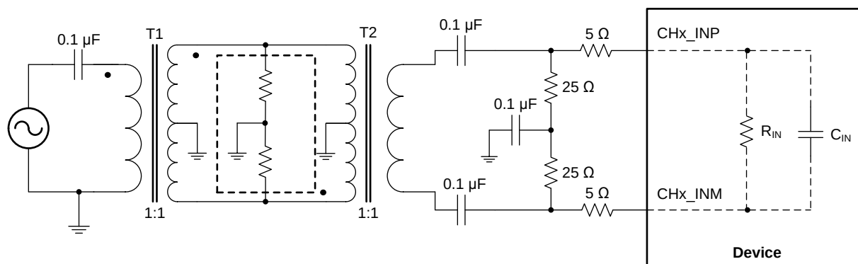
Figure 136. Input Drive Circuit
