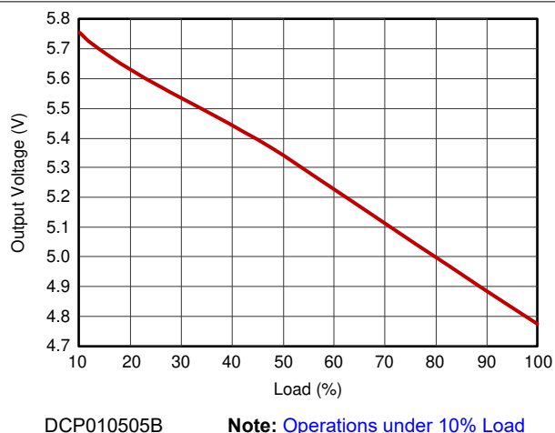
Figure 6-6. Load Regulation
