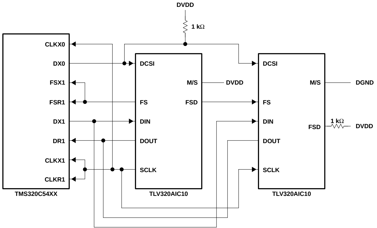
(a) Direct Configuration Between C54 and AIC10
