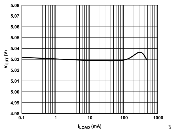
Figure 30. Output Voltage ( V_{OUT} ) vs. Load Current ( I_{LOAD} ), V_{OUT} = 5\text{ V} , Adjustable
