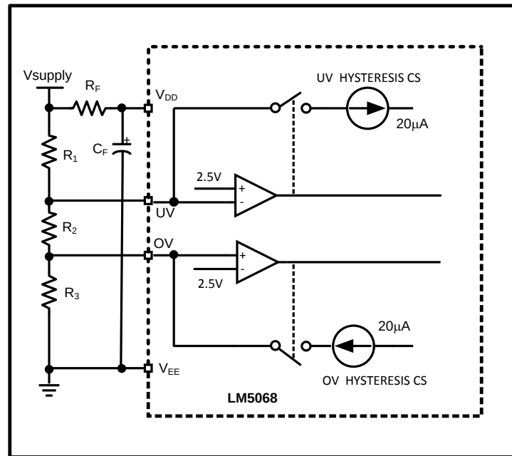
Figure 25. UV/OV Setting
