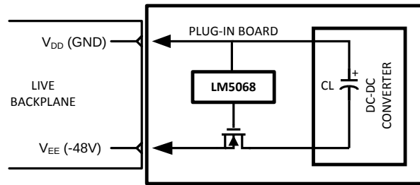
Figure 23. LM5068 Topology
