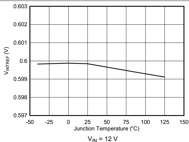
Figure 6-10. V_{INTREF} vs Junction Temperature
