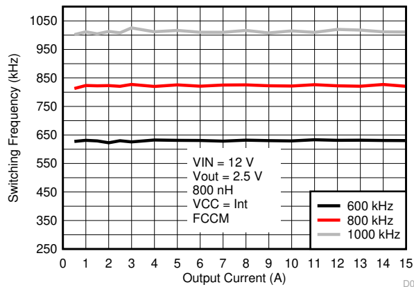
Figure 8-4. Switching Frequency vs Output Current
