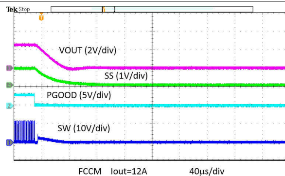
Figure 8-31. Over Temperature Protection in FCCM
