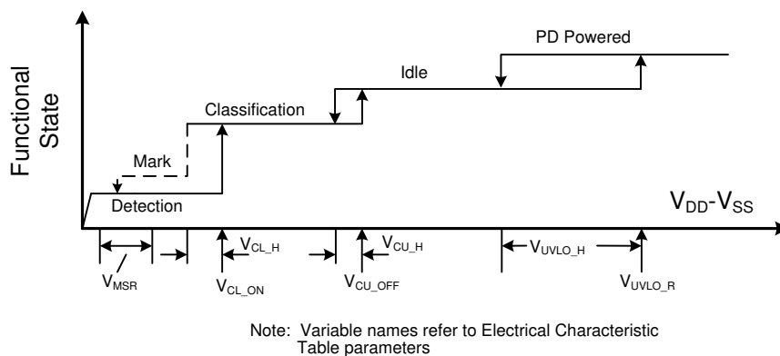
Figure 8-6. Threshold Voltages
