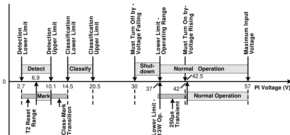
Figure 8-5. Operational States
