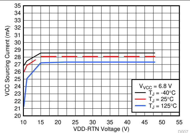
Figure 7-7. Converter Startup Current vs VDD Input Voltage
