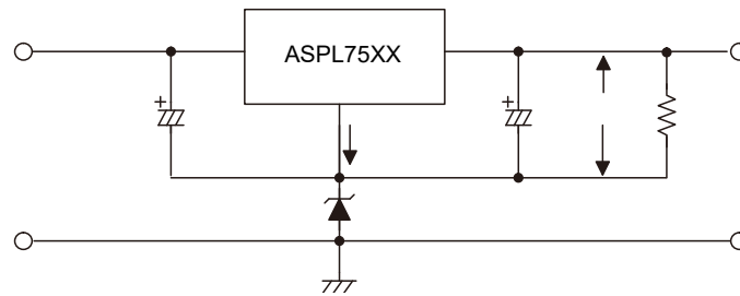
Circuit for Increasing Output Voltage
