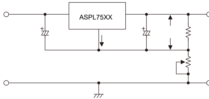
Circuit for Increasing Output Voltage
