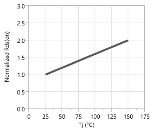
Figure 4. Normalized On-resistance
