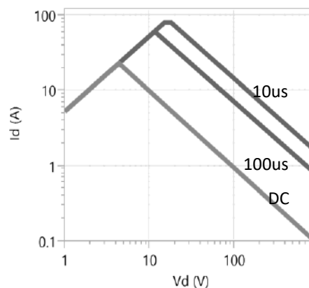
Figure 13. Safe operating Area T_c=80^\circ\text{C}
