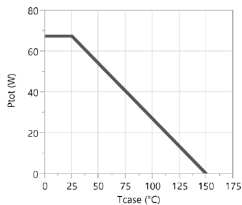
Figure 10. Power Dissipation
