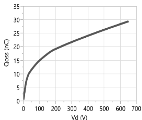
Figure 7. Typical Qoss
