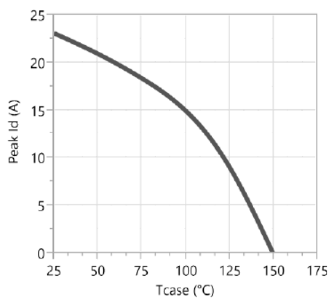
Figure 11. Current Derating
