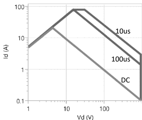
Figure 12. Safe operating Area T_c=25^\circ\text{C}
