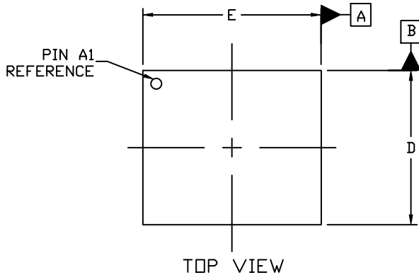
WLCSP87 2.643x3.053x0.354 CASE 567ZN ISSUE C
