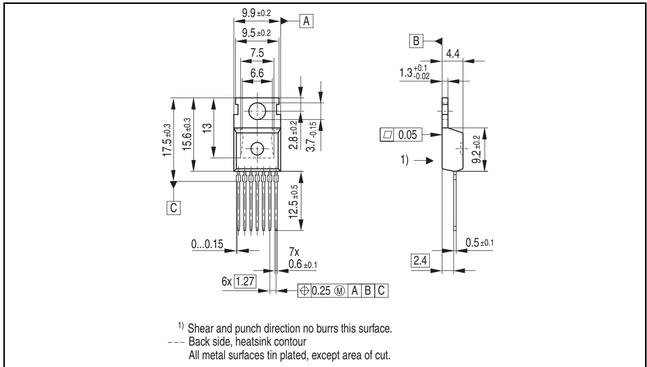
Figure 3 PG-TO220-7-230
