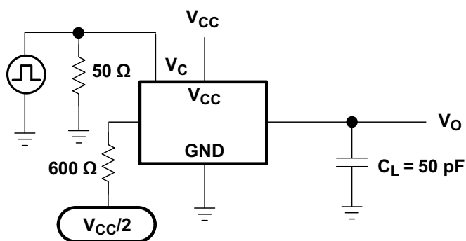
Figure 6-8. Crosstalk (Control Input – Switch Output)
