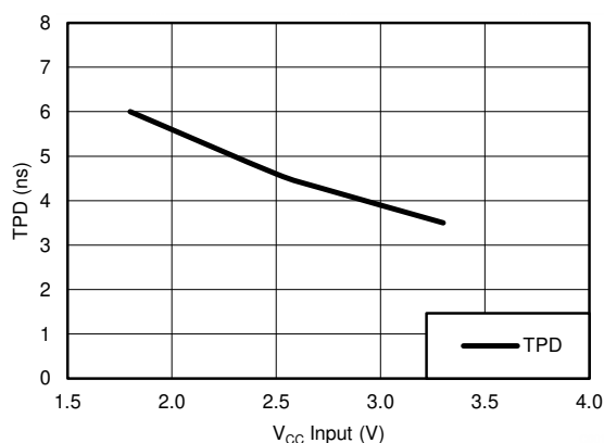
Figure 5-1. TPD vs V_{CC} ( T_A = 25^\circ\text{C} )
