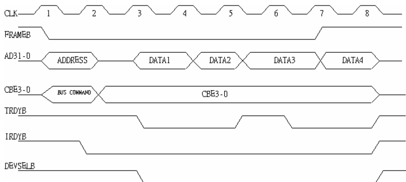
Figure 12. Memory Read
