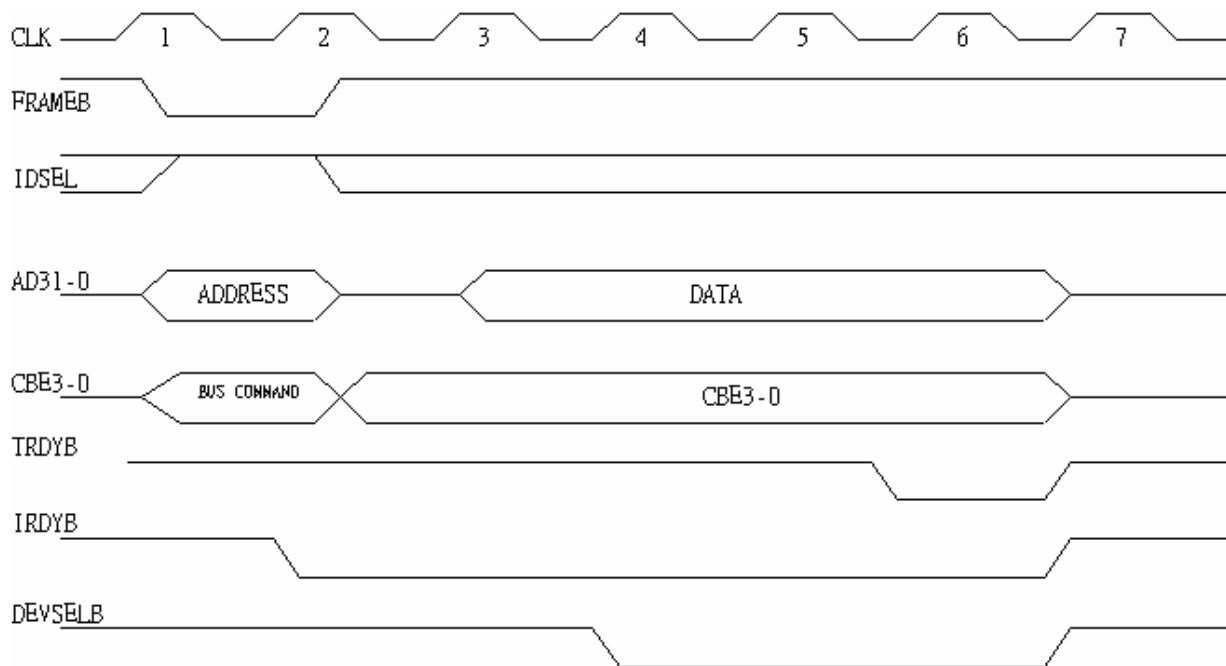
Figure 9. Configuration Read
