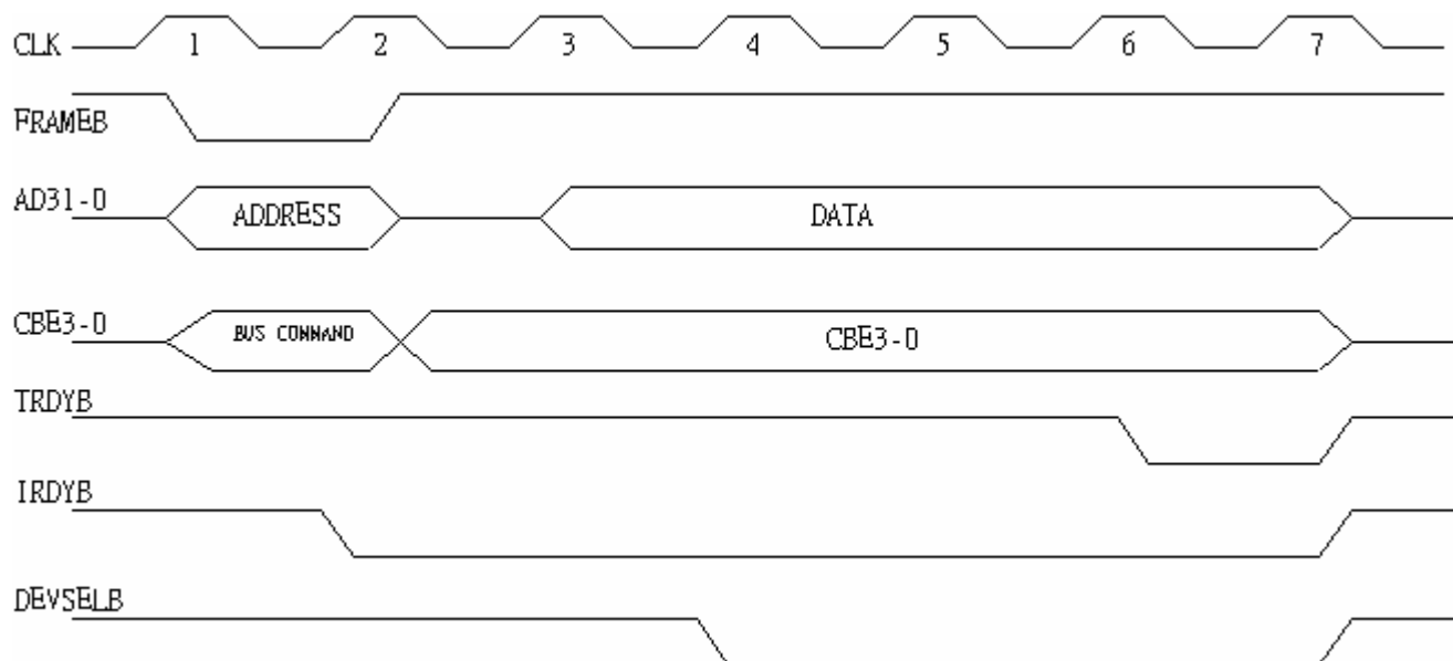
Figure 7. Target Read
