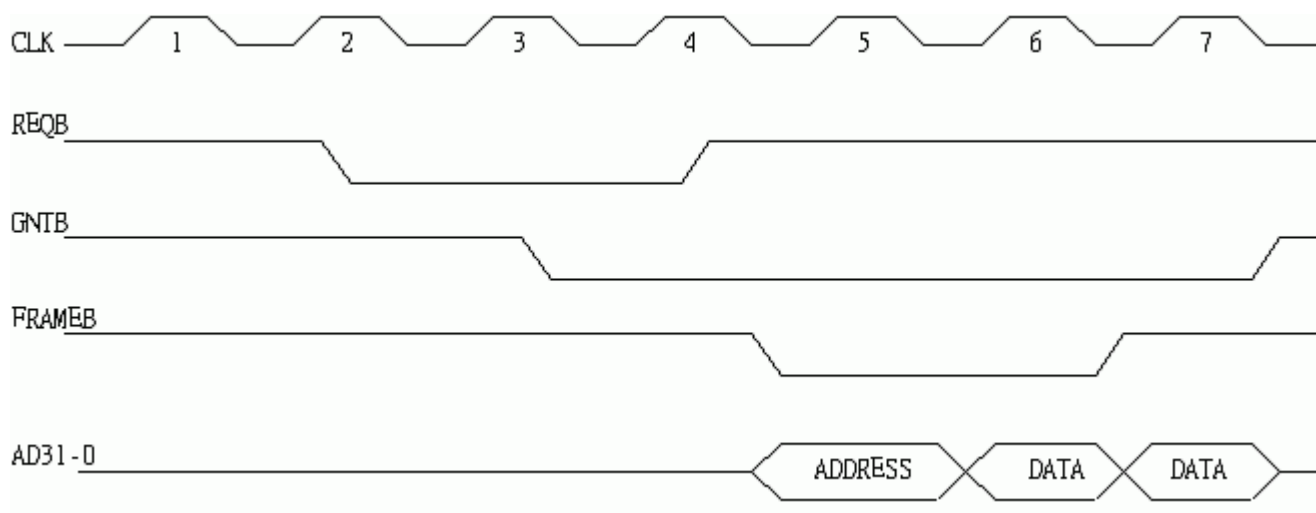
Figure 11. Bus Arbitration
