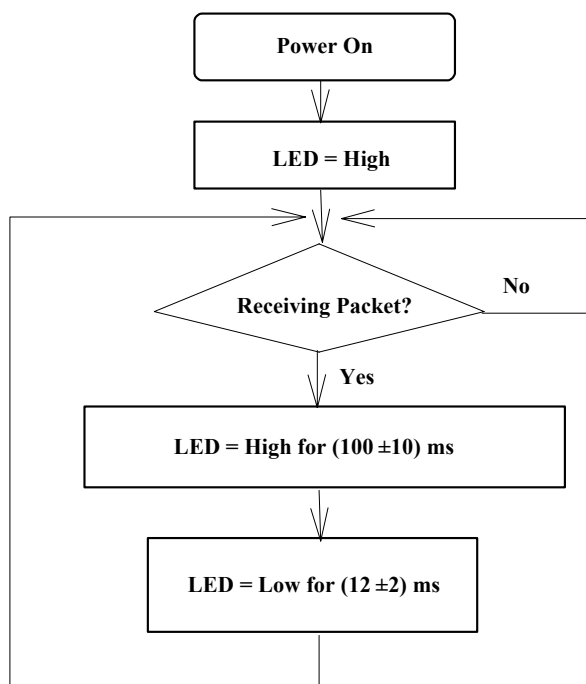
Figure 3. LED_RX
