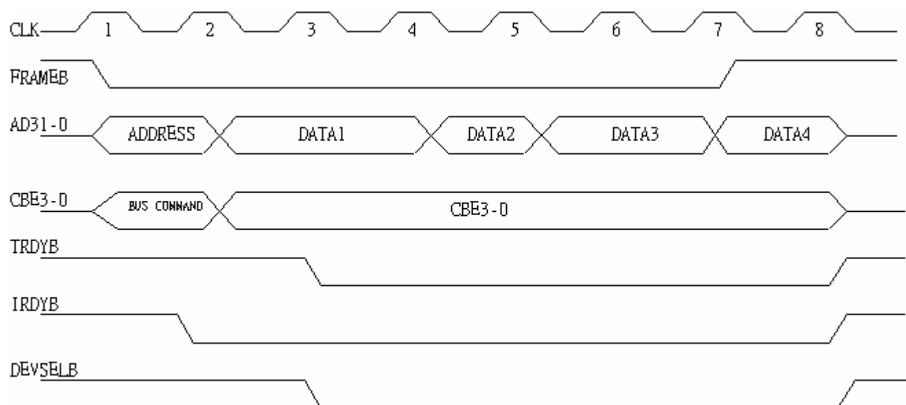
Figure 13. Memory Write
