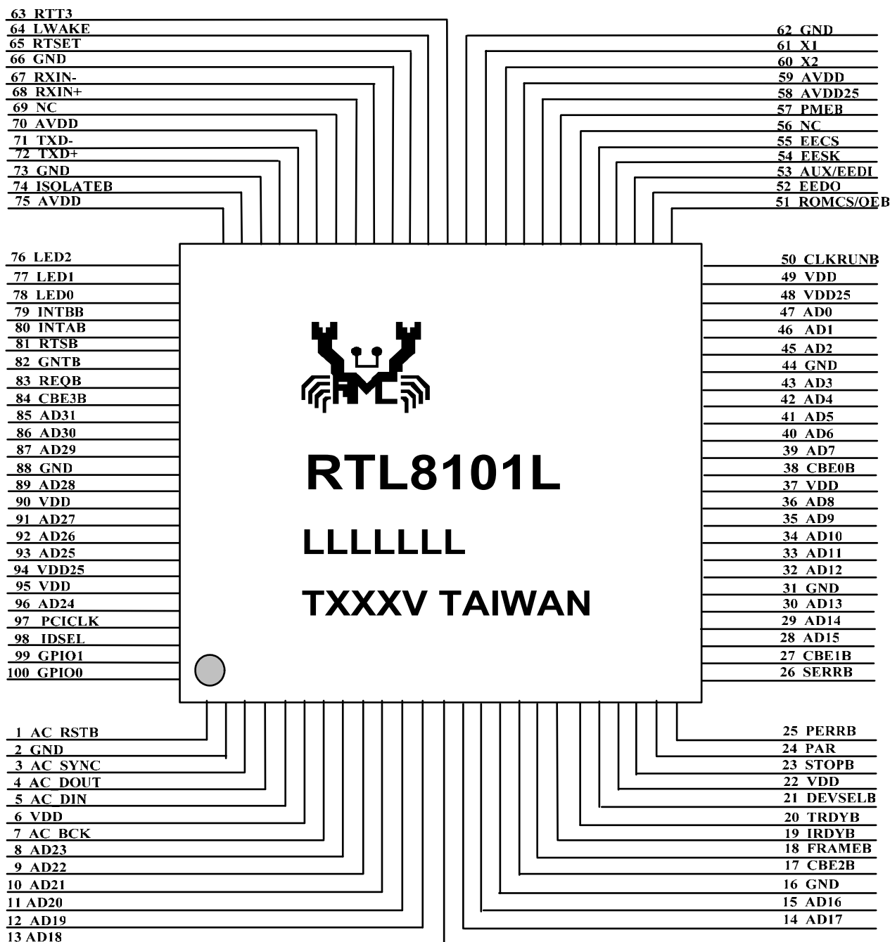
Figure 2. Pin Assignments
