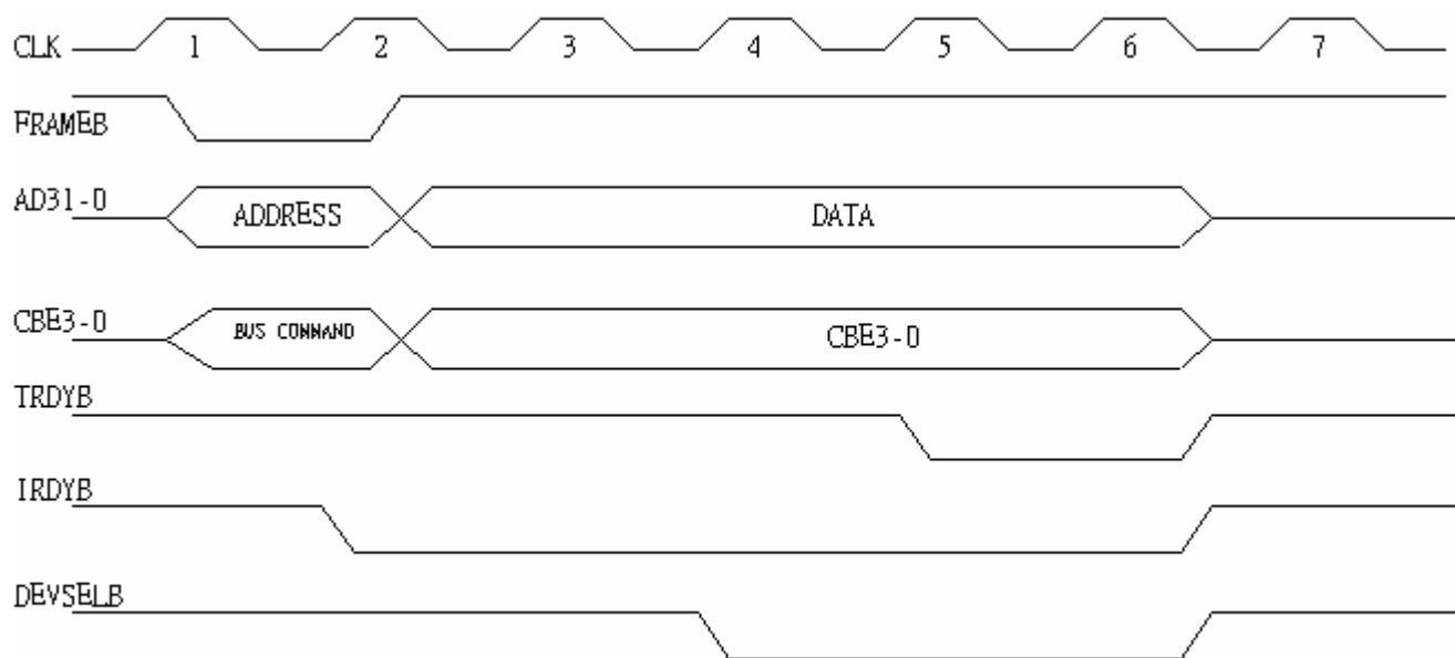
Figure 8. Target Write
