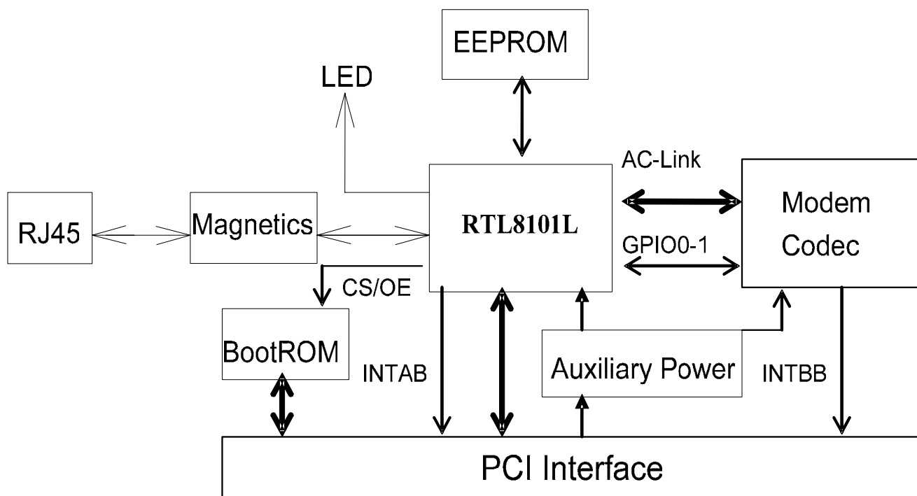
Figure 6. Application Diagram
