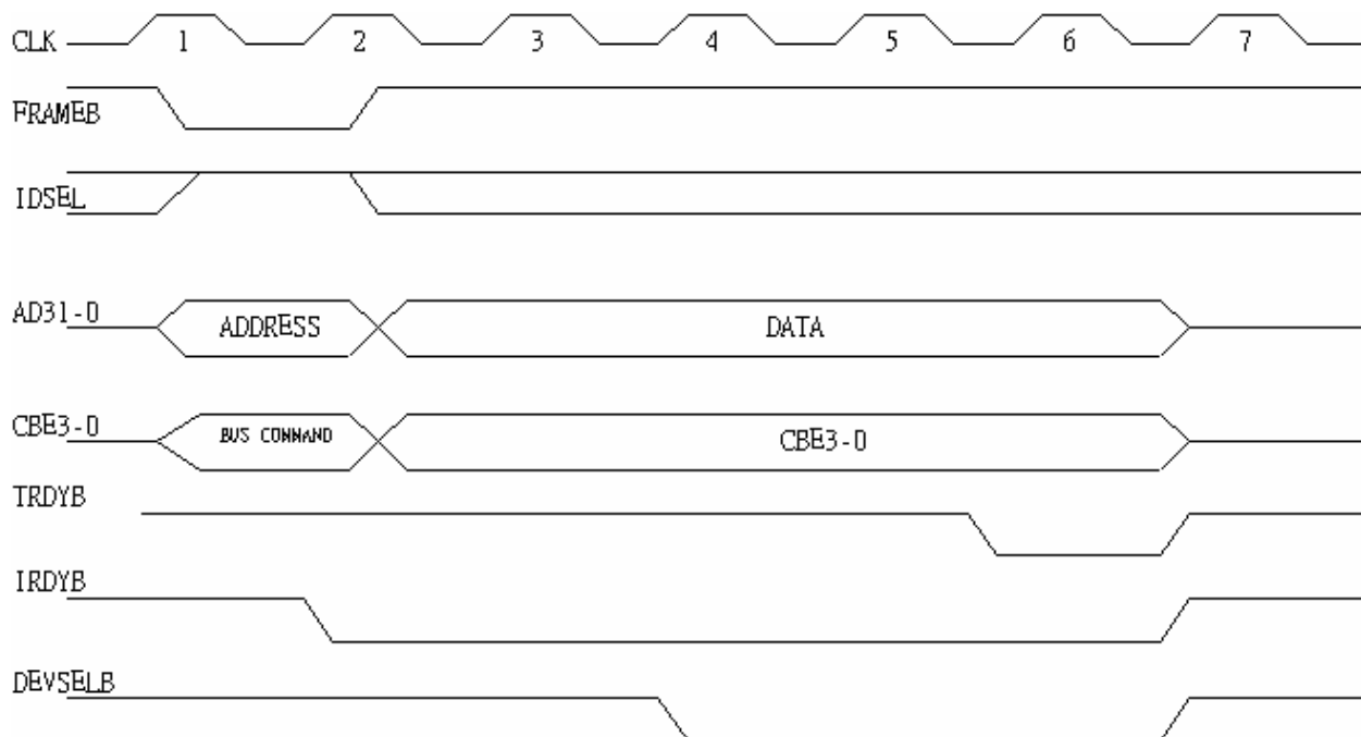
Figure 10. Configuration Write
