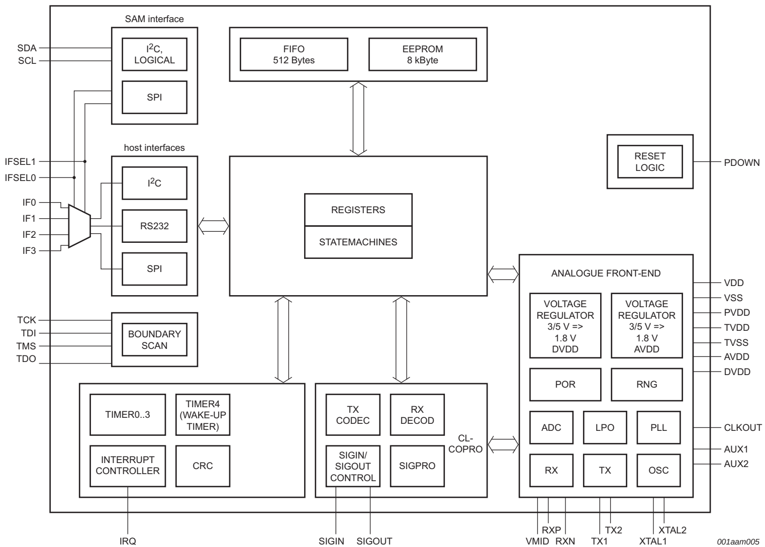
Fig 3. Detailed block diagram of the MFRC630
