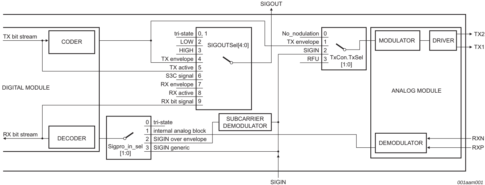
Fig 25. Overview SIGIN/SIGOUT Signal Routing
