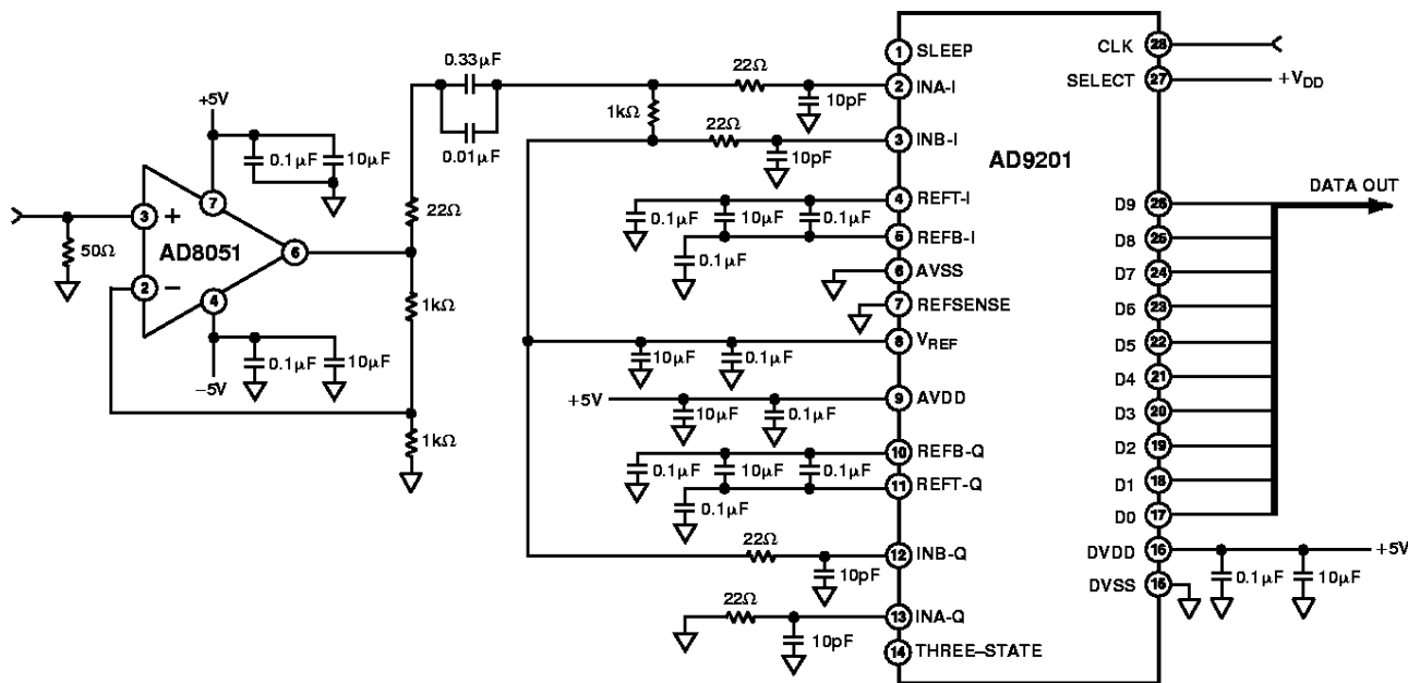
Figure 44. AD8051 Driving an AD9201, a 10-Bit 20 MSPS A/D Converter
