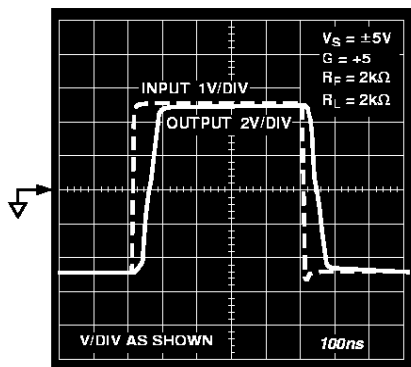
Figure 36. Overdrive Recovery
