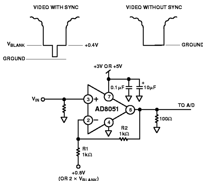
Figure 47. Sync Stripper
