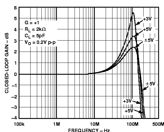
Figure 7. AD8054 Closed-Loop Frequency Response vs. Supply
