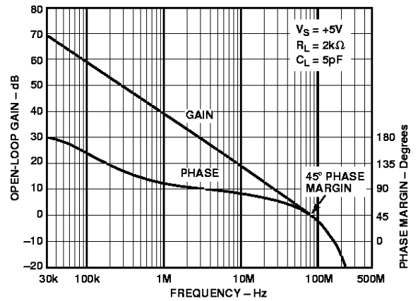
Figure 14. AD8054 Open-Loop Gain and Phase Margin vs. Frequency
