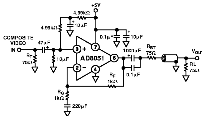
Figure 48. Single Supply Composite Video Line Driver
