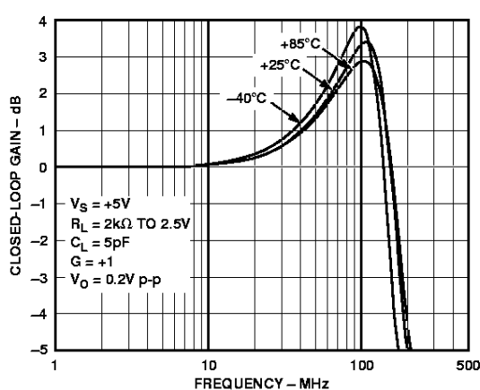
Figure 8. AD8054 Closed-Loop Frequency Response vs. Temperature
