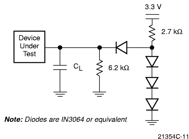
Figure 9. Test Setup
